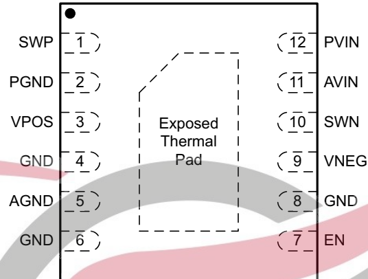
DPD Package 12-Pin WSON (Top View)
